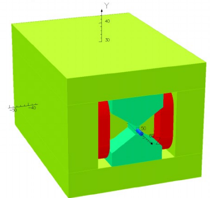
Magnet design
